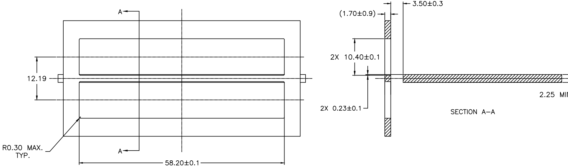
RECOMMENDED BEZEL DESIGN BELLY TO BELLY APPLICATIONS
