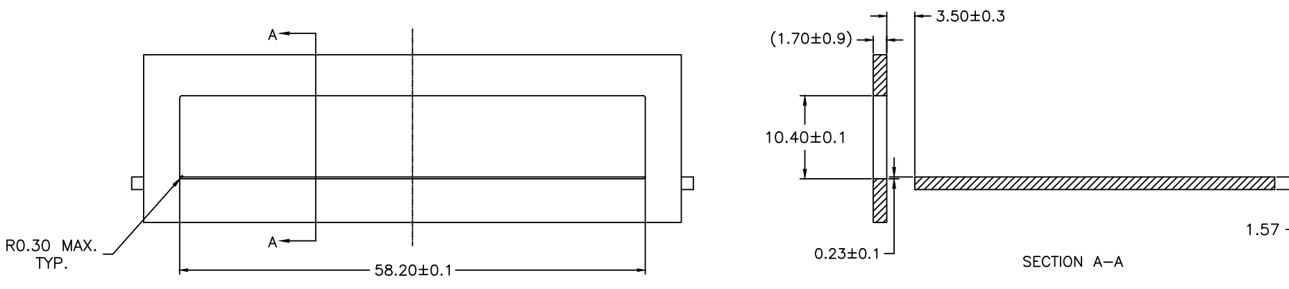
RECOMMENDED BEZEL DESIGN SINGLE SIDED APPLICATIONS
